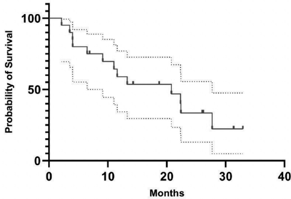
CUE-101 Survival Curve
